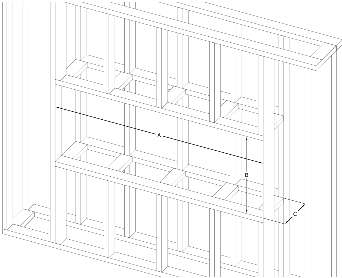
Figure 2.1 - Standard Installation Framing
