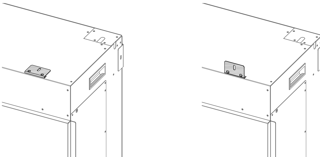
Figure 2.5 - Unfolding Nailing Flanges
